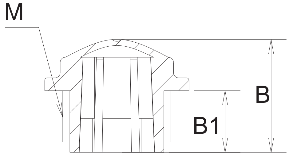
Sect. A-A
