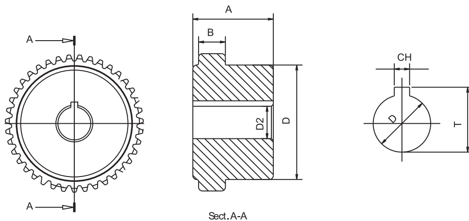
Sect. A-A
